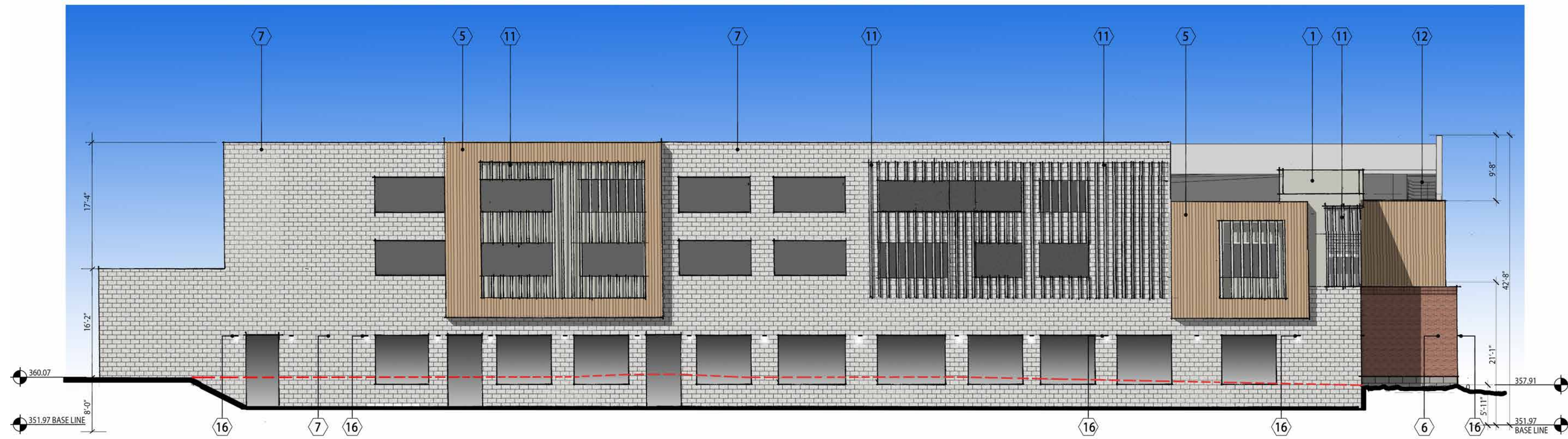
3 North Elevation 1/8"=1'-0"
