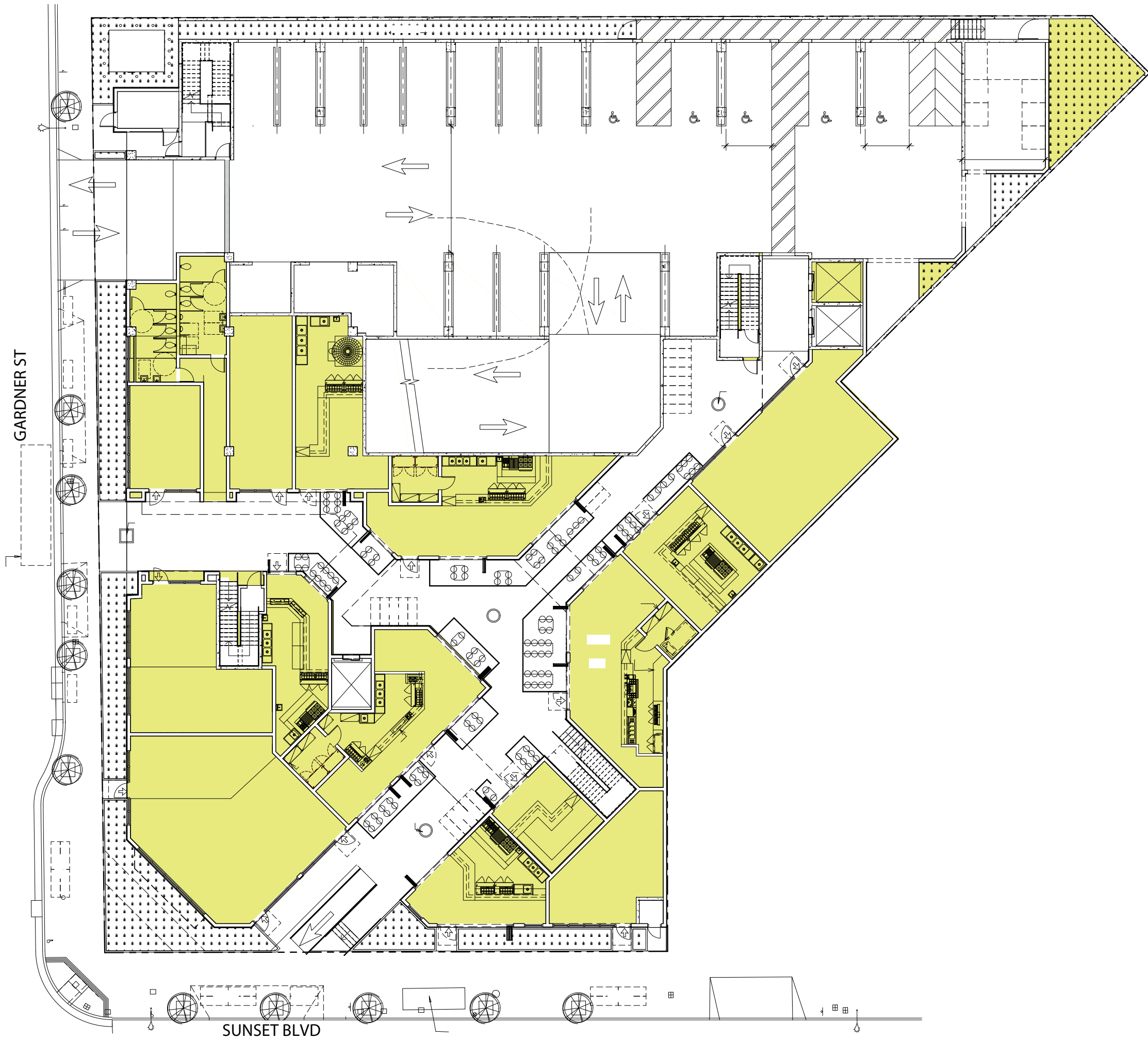
Key Plan 1
