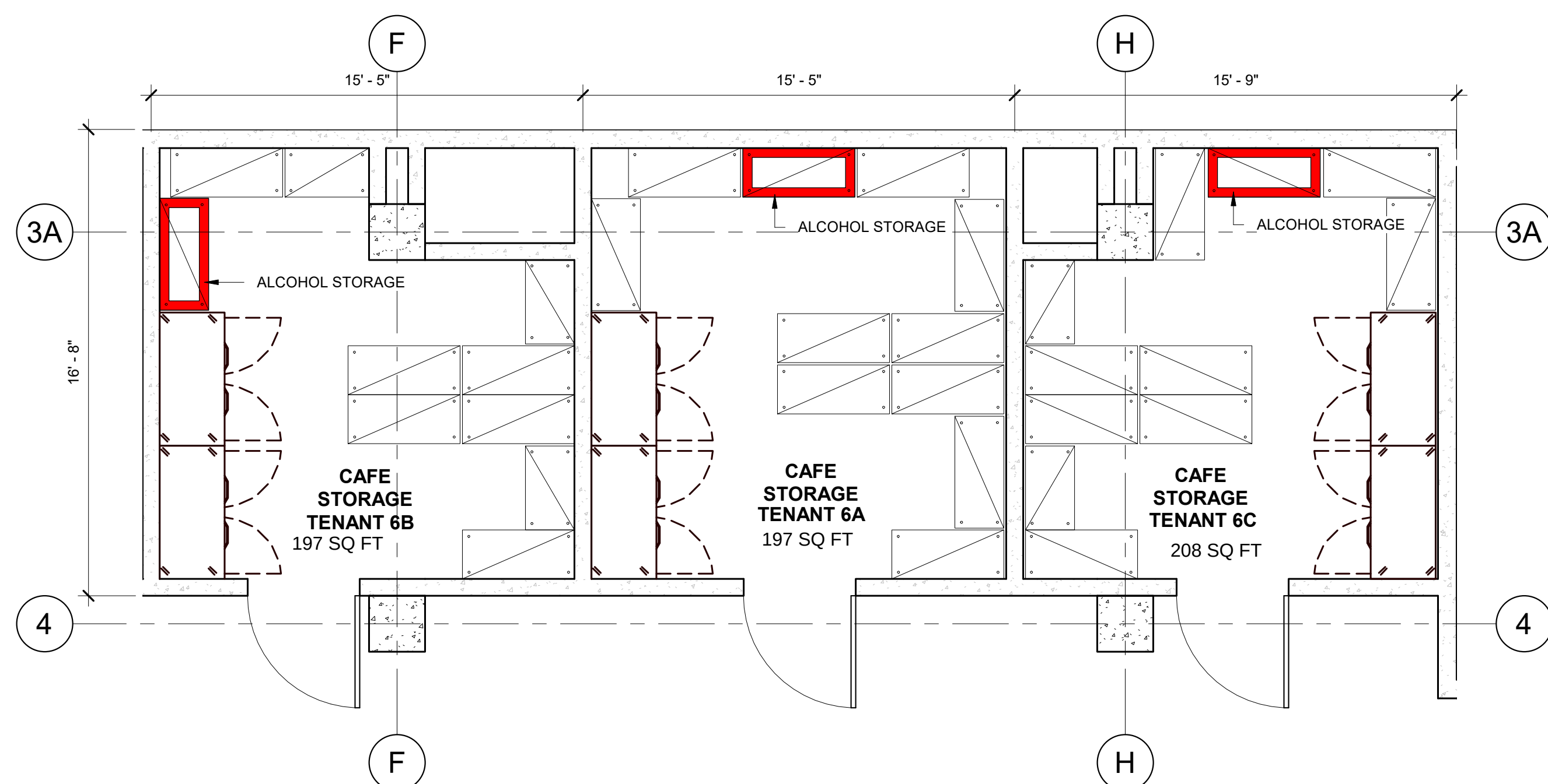
4 BASEMENT STORAGE FOR TENANT 6A, 6B, 6C 1/4" = 1'-0"
