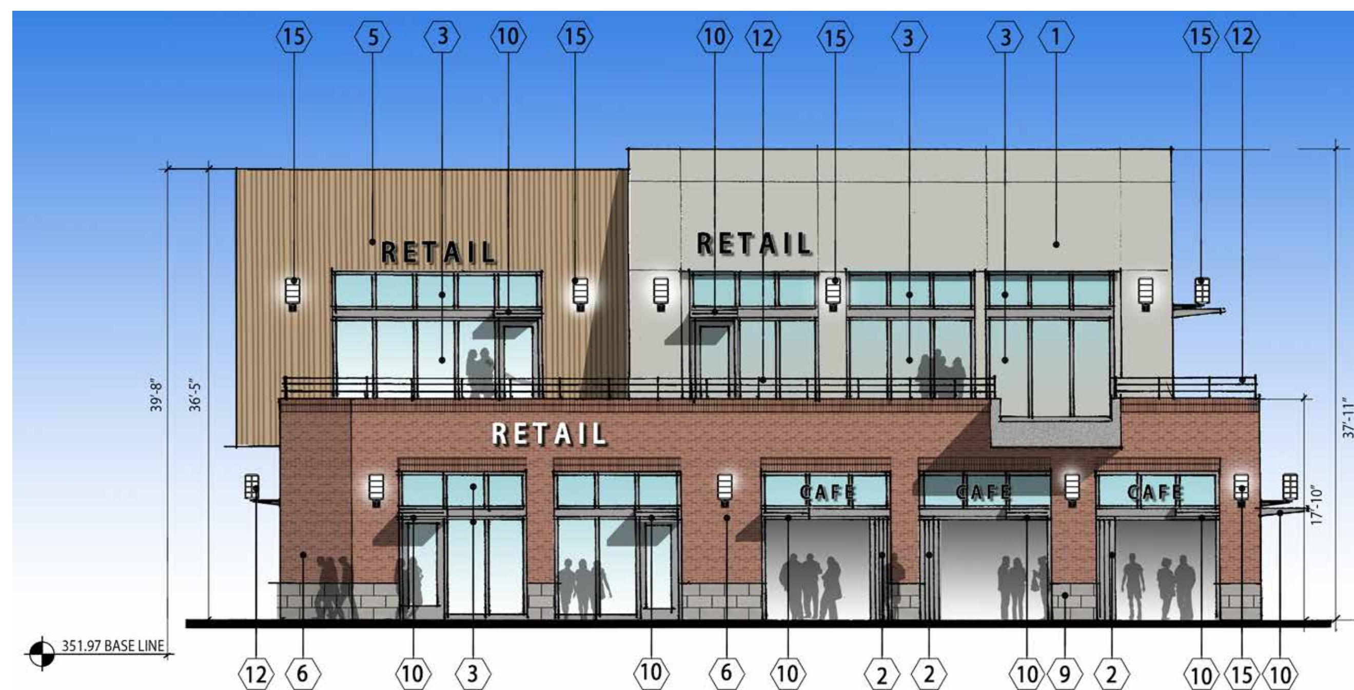
F2 Elevation 1/8"=1'-0"
