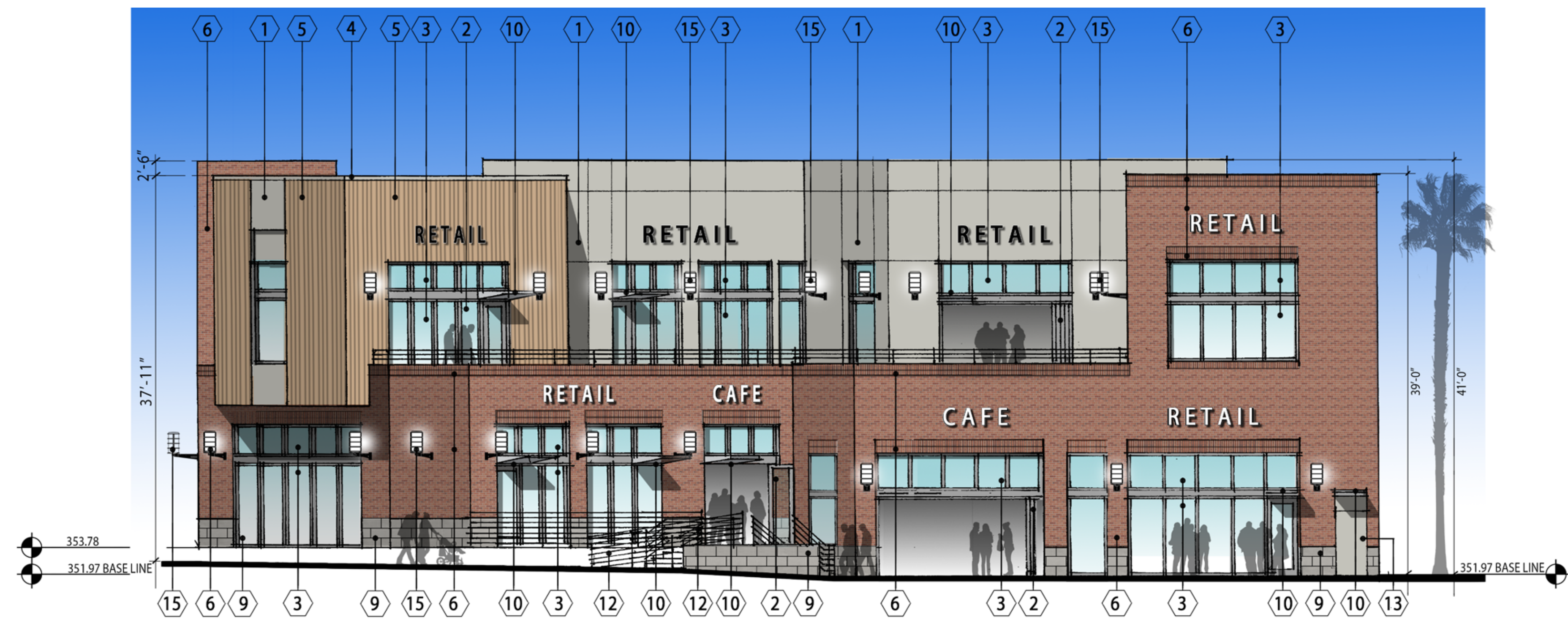
1 Sunset Blvd. Elevation 1/8"=1'-0"
