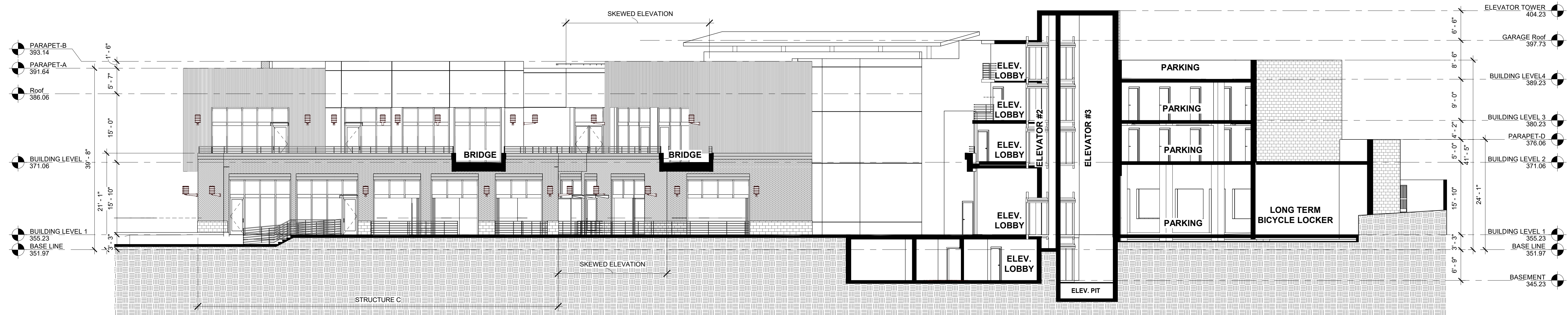
BUILDING SECTION C-C 3/32" = 1'-0"
